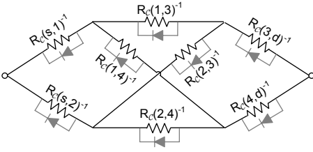
Fig. 2. The route subgraph G_n(s, d) in Fig. 1(a) is made non-planar by adding the edge (2, 3) . The resulting electric circuit \mathcal{E}_{sd} is illustrated.
