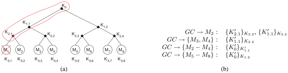
Fig. 1. (a) M_1 leaves the multicast group in a binary key tree, (b) Update messages sent by the GC to valid members.
