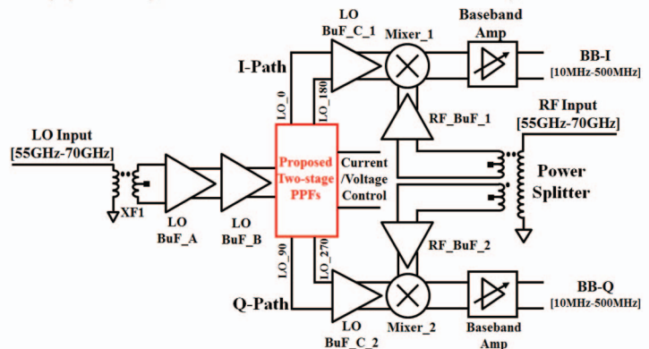
Fig.4 Block Diagram of the proposed system for IQ imbalance measurement
