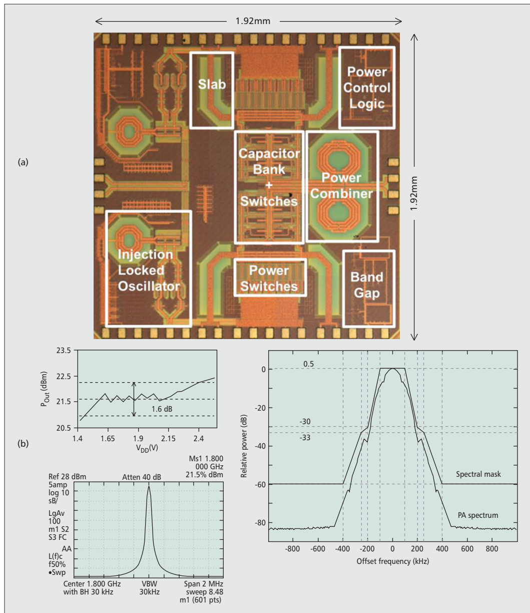
Figure 5. a) PA die photo; b) measurement results.
