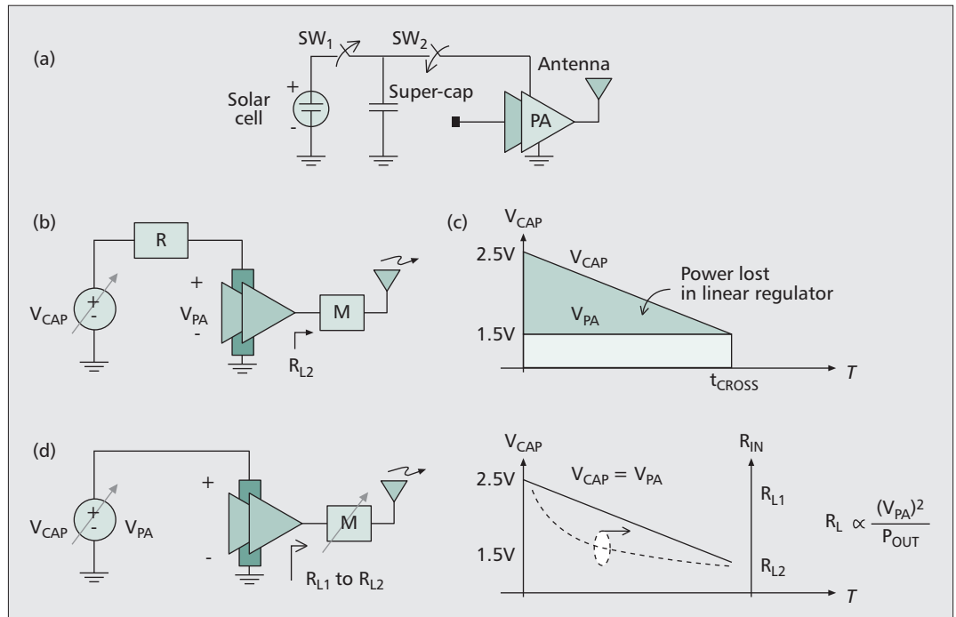
Figure 3. a) Simple energy scavenging device with super-cap, and transmitter; b) regulation of sensor energy source; c) conceptual plot of LDO losses in sensor systems; d) conceptual diagrams of regulator-less PA and tunable matching network.
