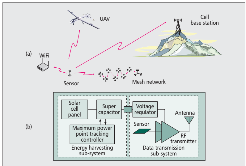
Figure 2. a) Long-range wireless sensor devices, and the potential for network scavenging; b) data transmission system (DTS).
