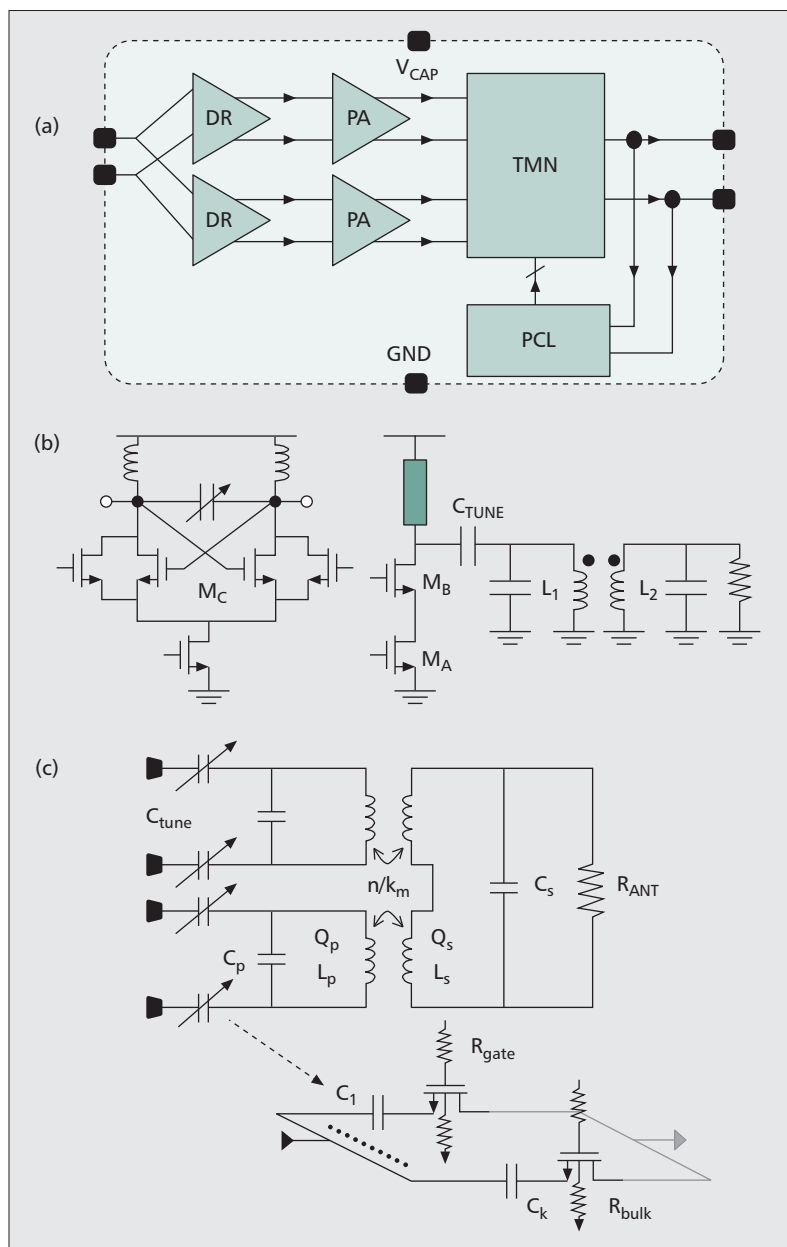
Figure 4. a) PA with tunable matching network (TMN) and power control loop (PCL); b) simplified schematic of PA first and second stages; c) power combining transformer with switch network.
