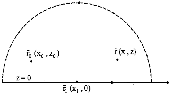
Fig. 2. Random integral equation (11).
