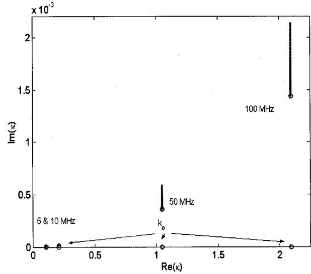
Fig. 7. Case 2: Zenneck wave propagation constant \kappa with k_o for increasing surface roughness \sigma = 0.0 – 0.2 m at 5, 10, 50, and 100 MHz.
