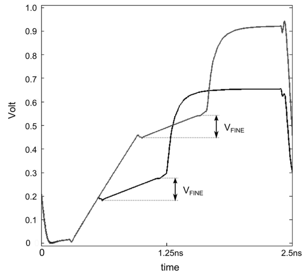
Fig. 14. Comparison of simulated output waveforms of small and large residues at V_{OUT+} .
